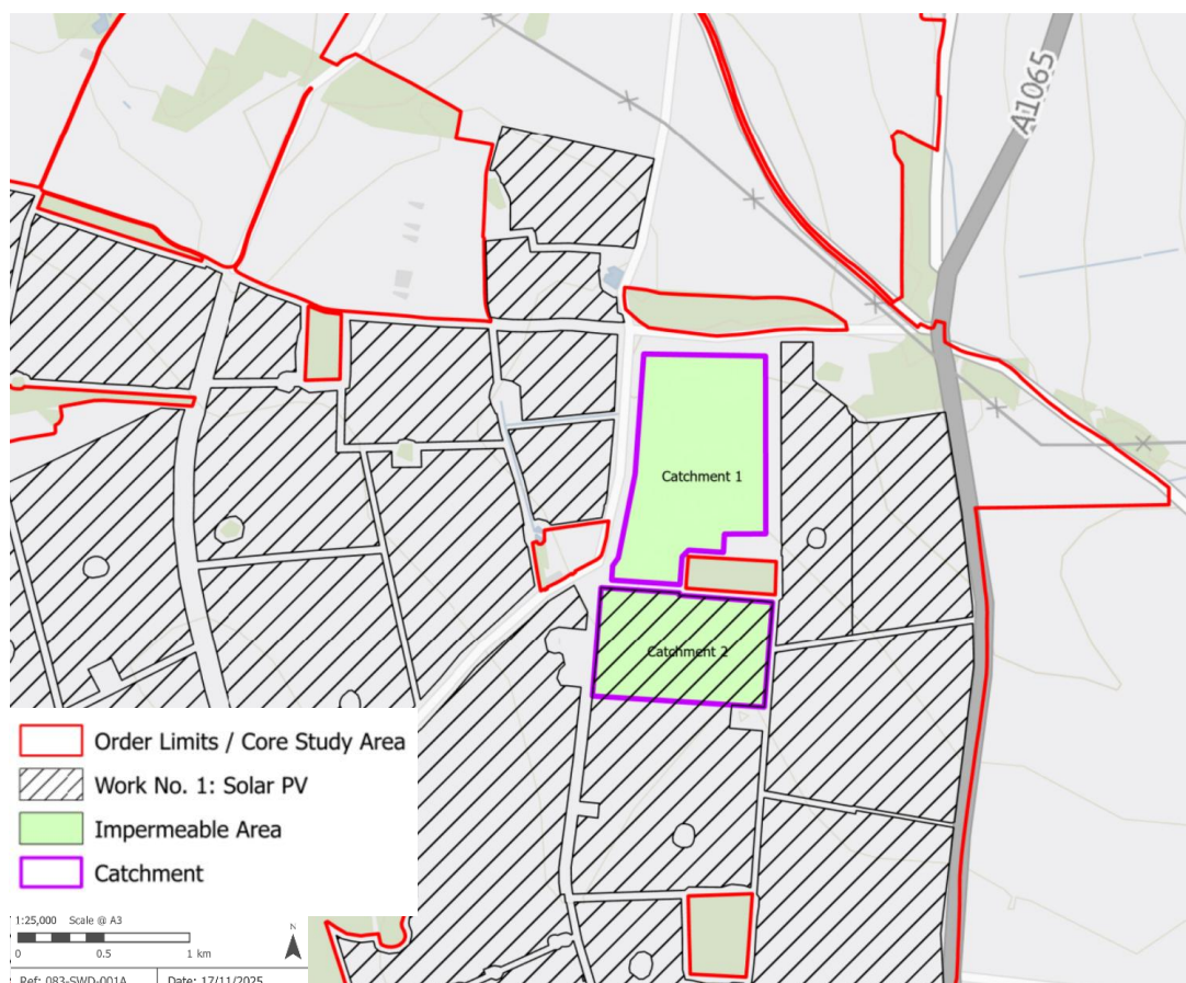
Plate 12-29 Contributing Catchments and Impermeable Areas
