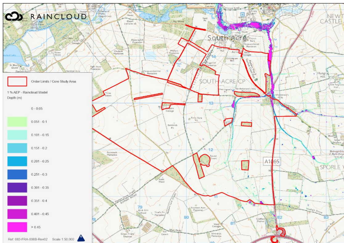
Plate 12-13 1% AEP Flood Depths – Raincloud 2D Modelling
