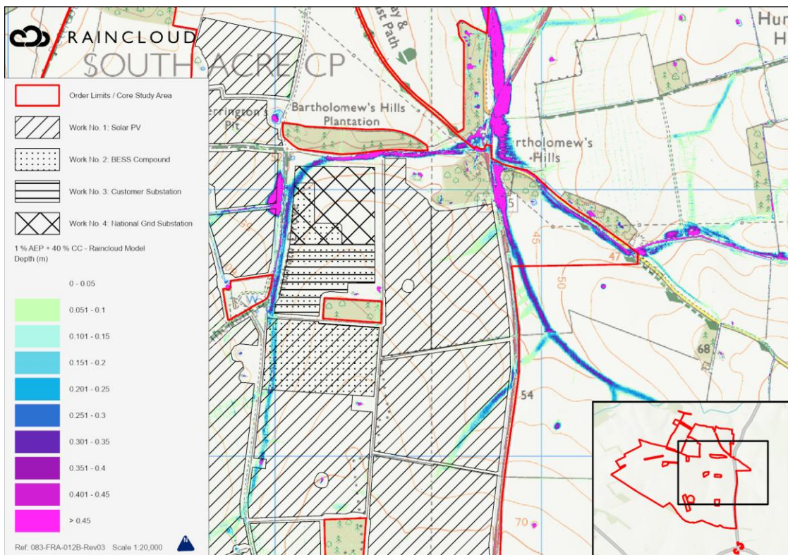
Plate 12-20 Modelled 1% AEP + 40% CC Pluvial Flood Depth
