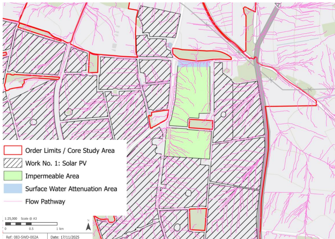
Plate 12-32 Exceedance Flow Pathways
